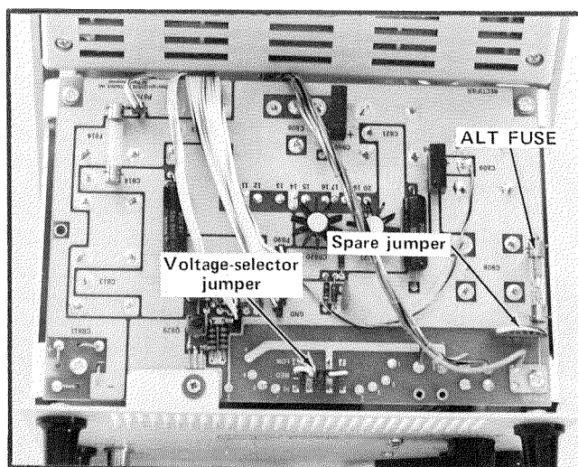
Fig. 1-1. Locations of voltage-selector jumper, spare jumper, and ALT FUSE in power unit (7603 shown).
