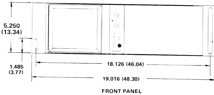
Fig. 3-6. Dimensional drawing.
