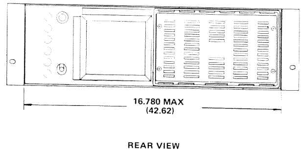
Fig. 3-6. Dimensional drawing.
